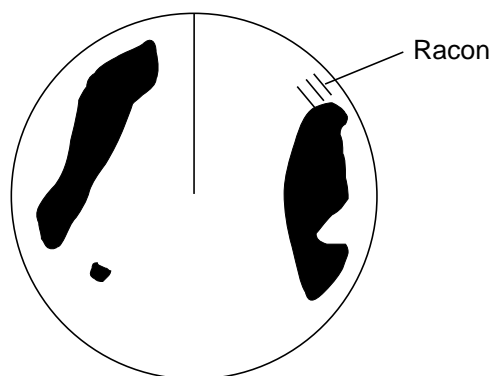
Figure 2-9 Appearance of RACON signal on the radar display
